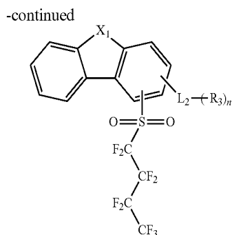
[Reaction Scheme 3]
