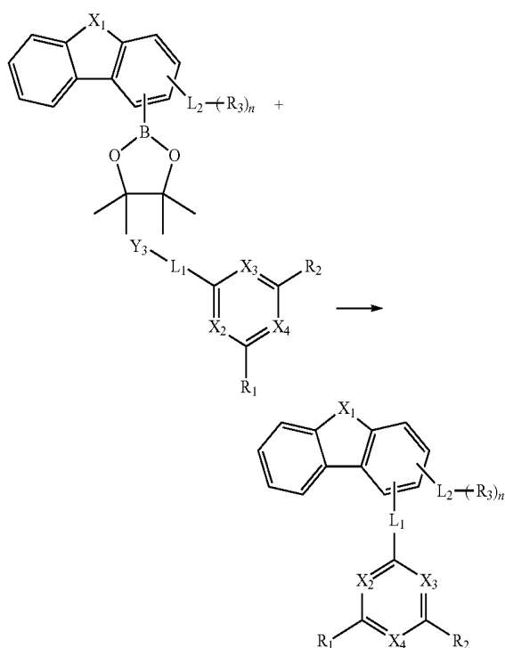
[Reaction Scheme 4]
