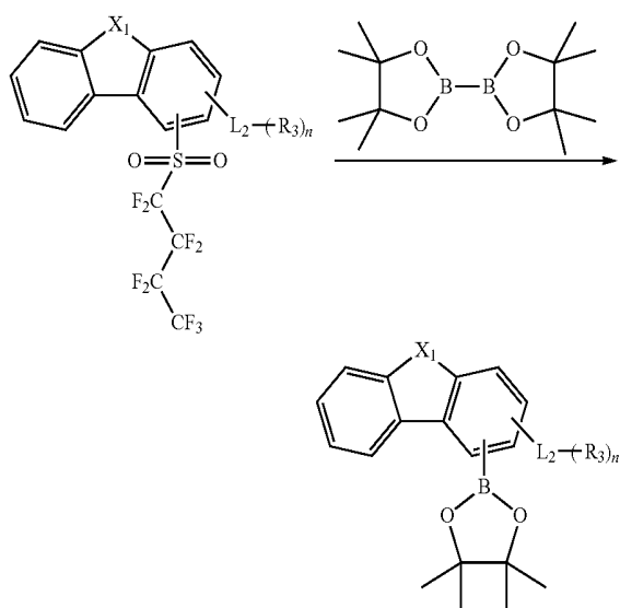
[Reaction Scheme 3]
